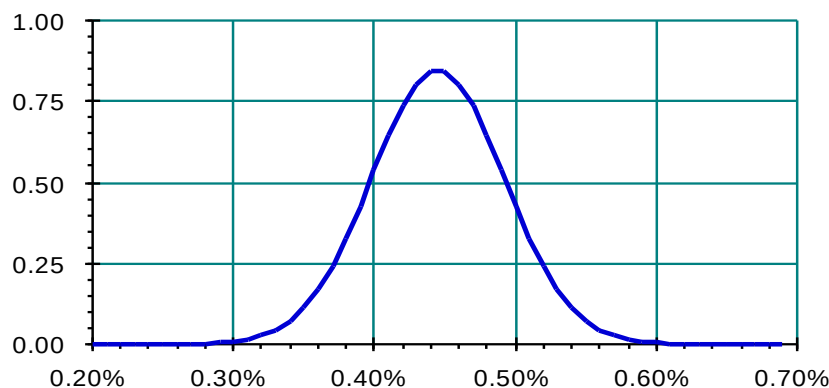
Figure VIII. 2 Gaussian distribution
