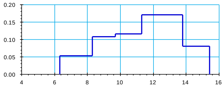
Figure VIII. 1 Discrete distribution
